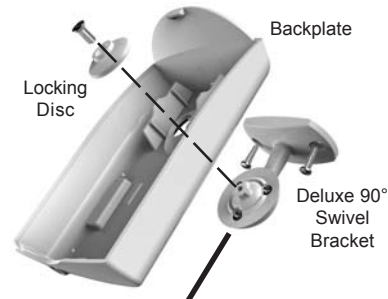
Figure 8. Deluxe 90° Swivel Bracket (Separate purchase P/N: ELK-603022)
