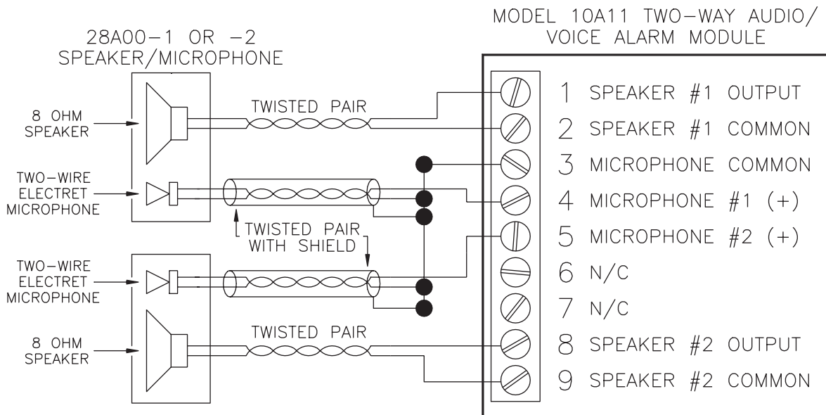
FIGURE 1 – Speaker/Microphone Connections
