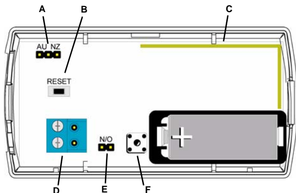
Figure 1 Transmitter components
