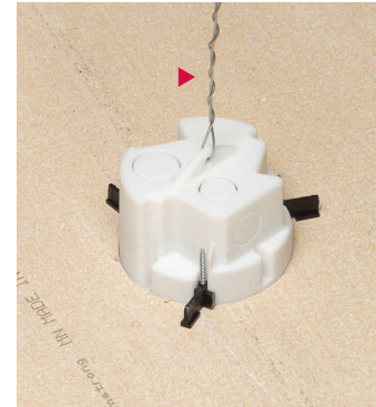
3 Wrap drop wire twice through loop on top of box and around a framing member above ceiling. Wrap wire around itself six times minimum in both instances.
