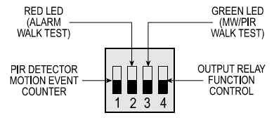
Figure 5. DIP Switch Mode Selector
