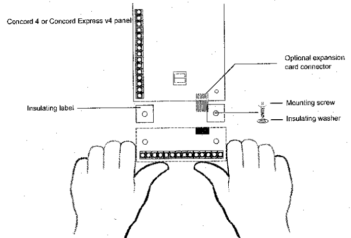
Figure 1. SnapCard installation
