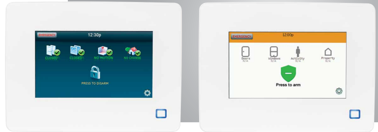
Classic interface
