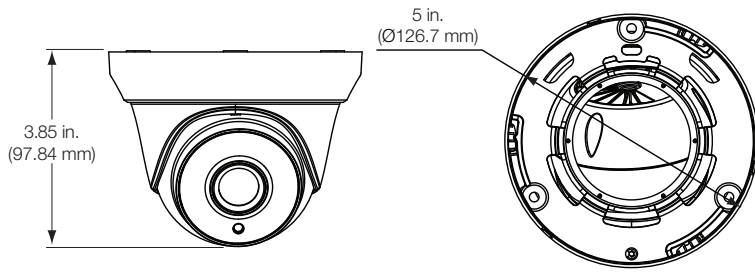
TVT-4402, TVT-2402, TVT-4404, TVT-2404 Motorized Varifocal Turret Camera (adapter plate included)
