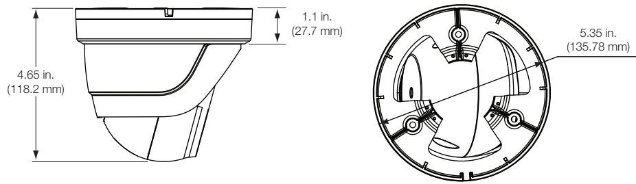
TVT-4402, TVT-2402, TVT-4404, TVT-2404 Motorized Varifocal Turret Camera (adapter plate included)
