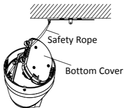
Figure 2-7 Hook the Camera to the Adapter
