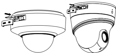
Figure 2-7 Insert the Memory Card
