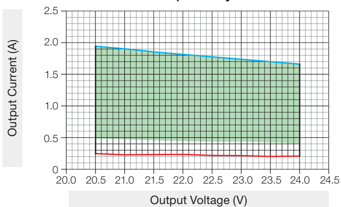
Load Compatibility
