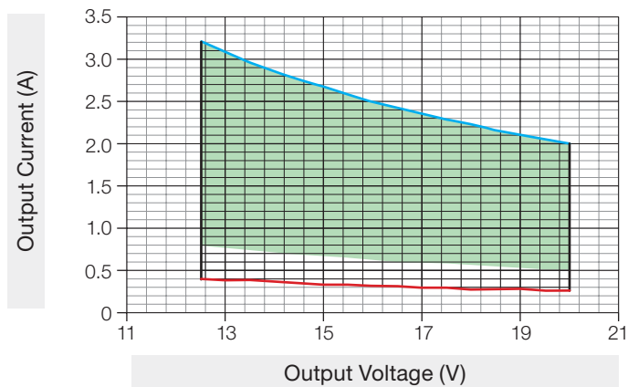
Load Compatibility
