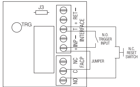
Fig. 8 Normally Open FACP Latching trigger input with reset (This output has not been evaluated by UL):
