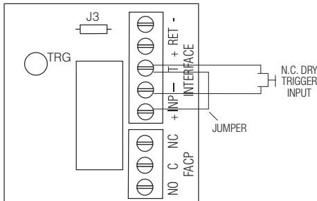
Fig. 9 Normally Closed: Non-Latching FACP trigger input:
