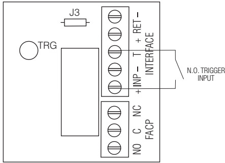
Fig. 7 Normally Open: Non-Latching FACP trigger input:
