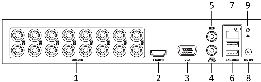
Figure 1-22 Rear Panel of DS-7200HQHI-K1/E
