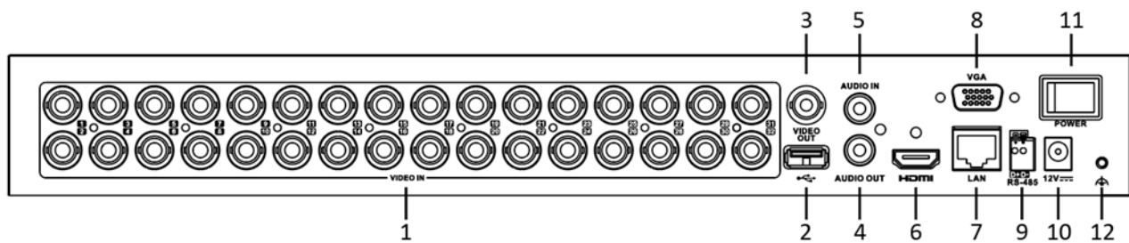
Figure 1-33 Rear Panel of DS-7200HGHI-K2
