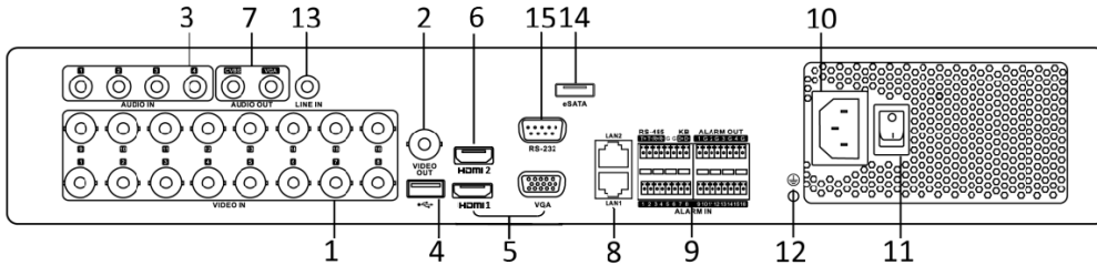
Figure 1-25 Rear Panel of DS-7300HUHI/HTHI-K4 and iDS-7316HUHI-K4/16S
