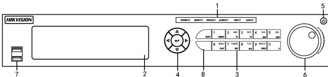
Figure 1-2 Front Panel
