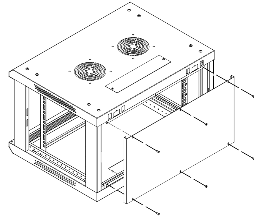
(3) Assembly the back panel by 6pcs M4*8 self- tapping screws.
