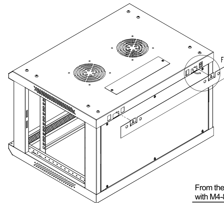
(4) Assembly the mounting bracket by 2pcs M4*8 selftapping screws.
