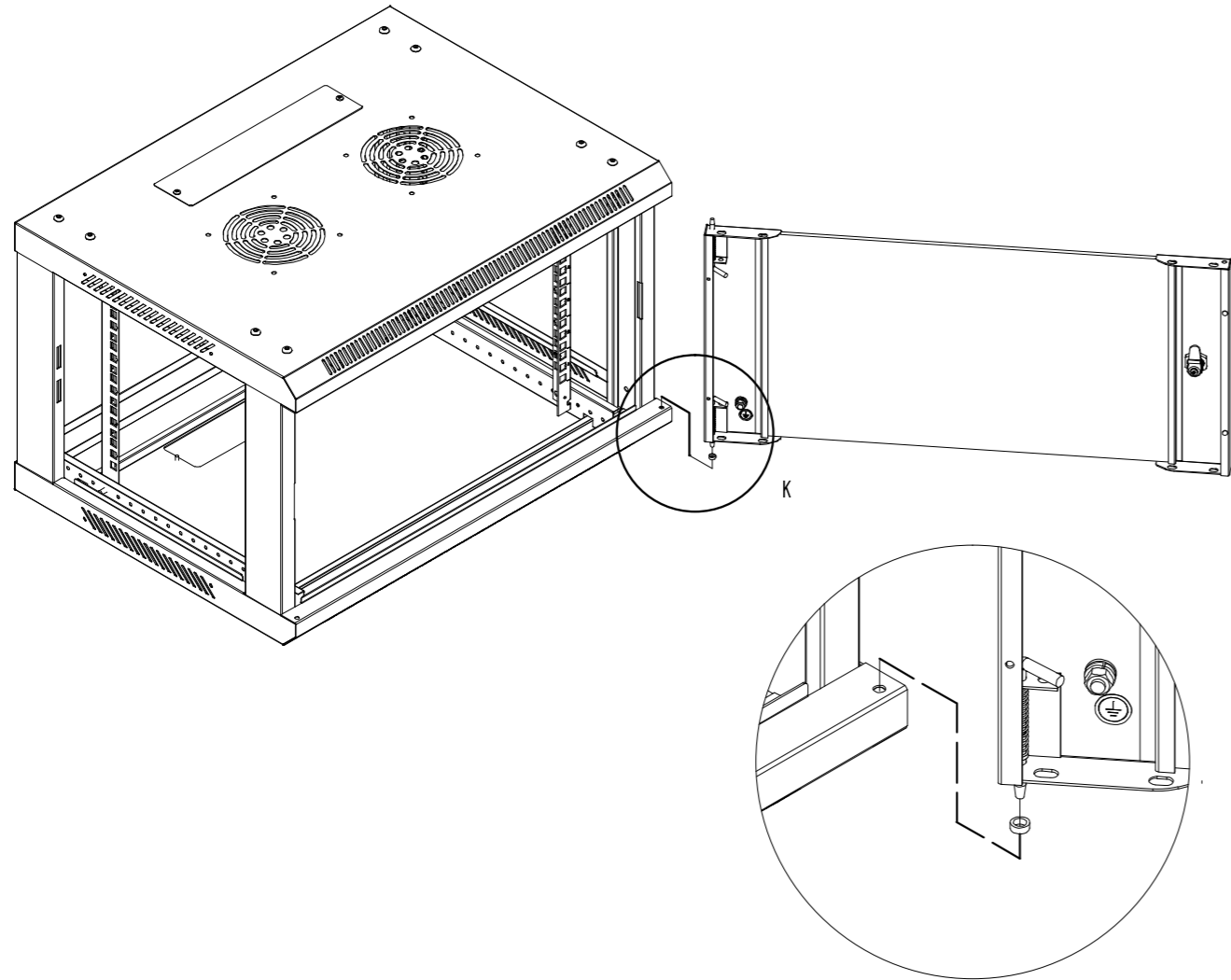
The local view K Proportion 2:1
