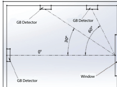
Figure 3. Angle between detector and window
