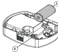
Figure 6. Battery Insertion
