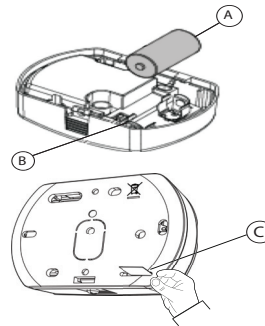
Figure 5. Inside View
