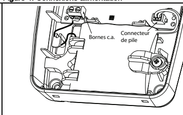
Figure 4: Connexions alimentation
