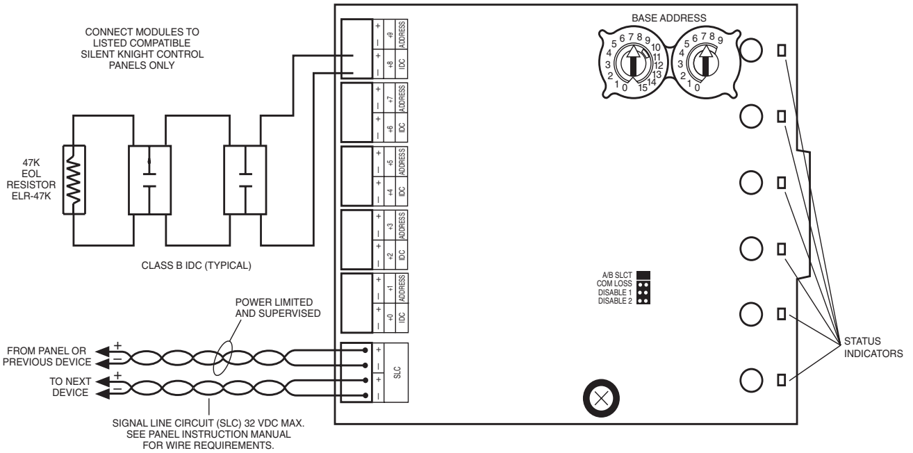
FIGURE 5: TYPICAL INITIATING DEVICE CIRCUIT CONFIGURATION – CLASS B, STYLE B.
