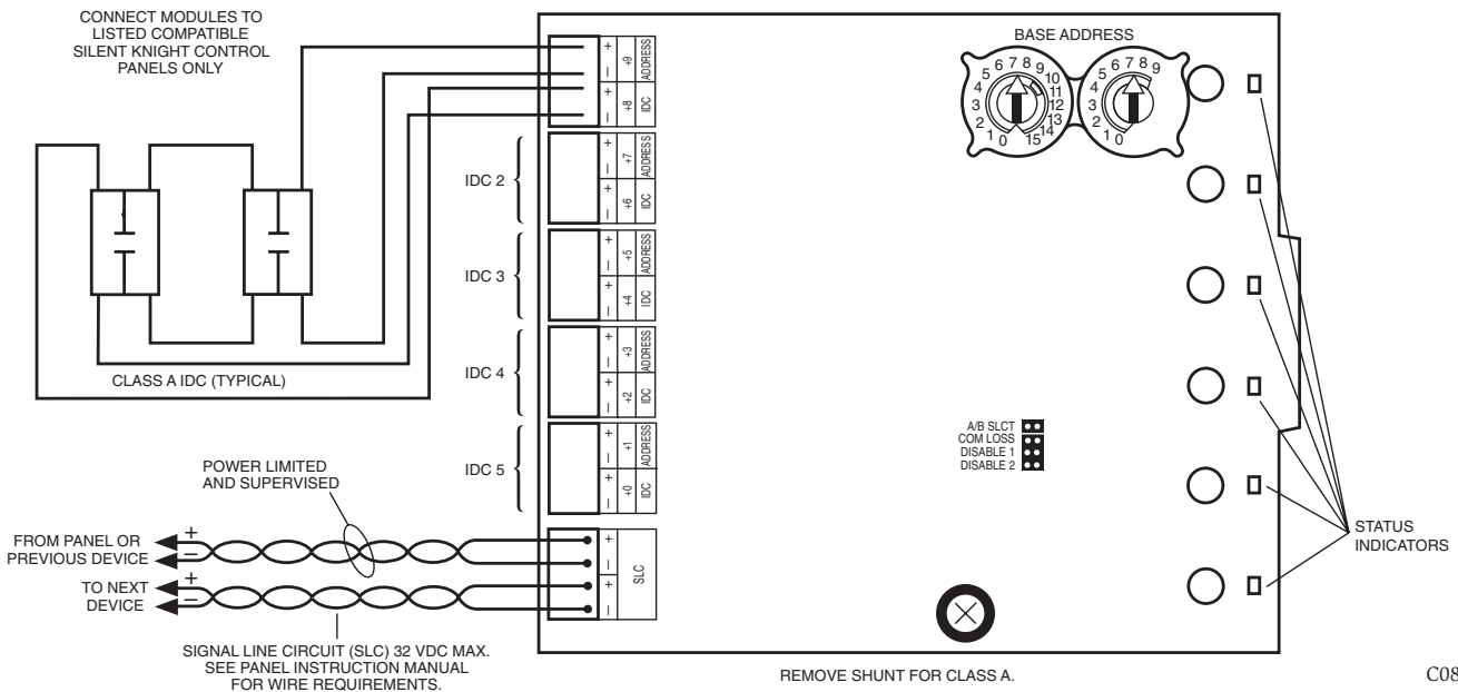
FIGURE 6: TYPICAL FAULT TOLERANT INITIATING DEVICE CIRCUIT CONFIGURATION – CLASS A, STYLE D
